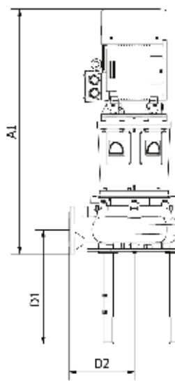
DanPumps S-WN3 - Vertikal installation
